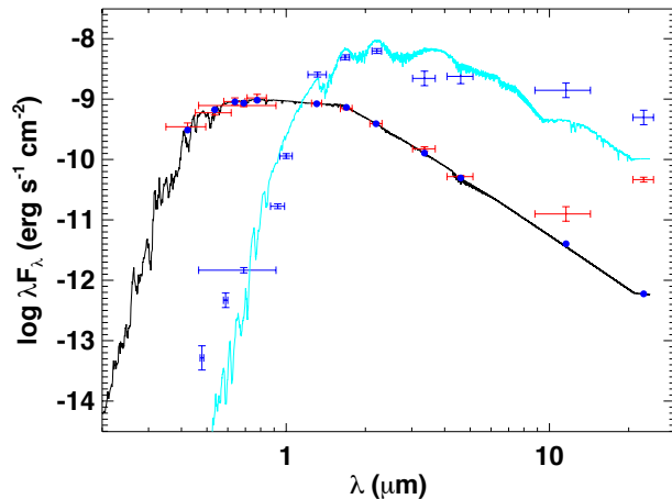
Figure 3. Best fit spectral energy distribution (SED) for TOI-824. Red symbols represent the observed photometric measurements, where the horizontal bars represent the effective width of the passband. Blue symbols are the model fluxes from the best-fit NextGen atmosphere model, which is shown in black. A fit to the infrared-bright source separated by \sim 25'' is represented by dark blue symbols and a cyan model. Note that the W3 and W4 bands (the two reddest) for TOI-824 were not used in the SED fitting, and the companion was ignored.
