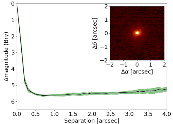
Figure 2. VLT/NaCo contrast curve and image (inset) for TOI-824. Images were taken with a \text{Br}\gamma filter and reach a contrast limit of 5 mag at 250 mas. No visual companions are detected anywhere in the field of view.
