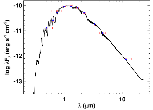
Fig. 4. SED of TOI-2257. The red symbols represent the observed photometric measurements; the horizontal bars represent the effective width of the passband. The blue symbols are the model fluxes from the best-fit NextGen atmosphere model (black).
