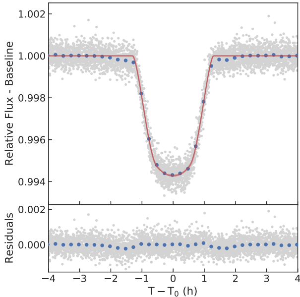
Figure 9. Phase-folded and detrended TESS multi-scale MAP PDC light curve of TOI-1431 (Sectors 15 and 16) from the simultaneous hybrid cubic spline detrending model, focusing on the transit. Systematics and other quality-flagged data (as shown in Figure 1) that are the result of, for example, spacecraft pointing anomalies have been removed prior to performing the analysis on the light curve. The blue points are binned at a cadence of 15 m and the red solid lines are 20 light curve models drawn from the posteriors of the Markov Chain Monte Carlo (MCMC) analysis in Allesfitter . Dip features starting \sim 1 hr before and after transit ingress and egress, respectively, are apparent in the light curve and were introduced during the PDC multi-scale MAP cotrending process. These dip features are not present in the single-scale MAP corrected PDC and SAP versions of the light curve (see Figure 10).
