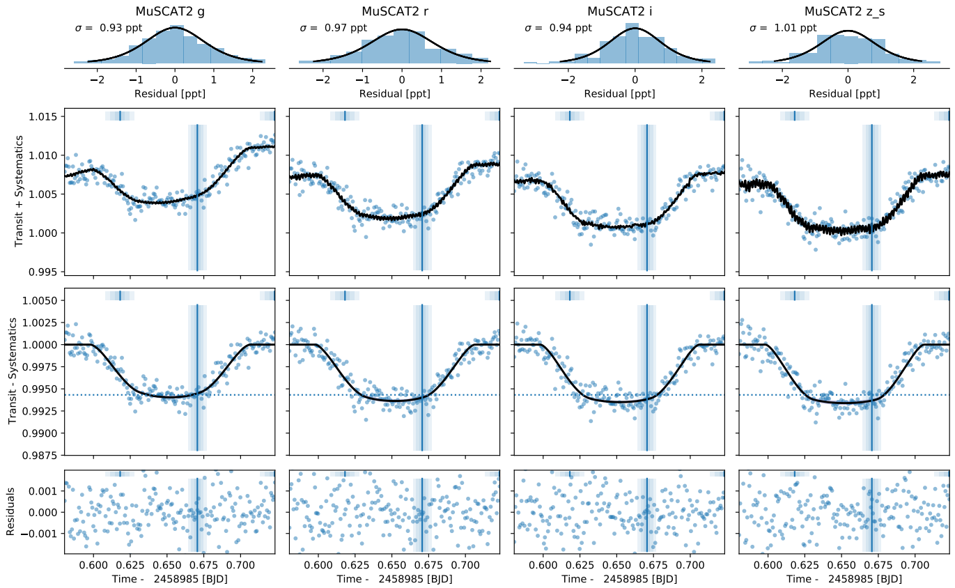
Figure 14. An observed transit on 16 May 2020 by MuSCAT2 using simultaneous multi-color photometry in g' , r' , i' , and z_s bands. The top panel shows the distribution of residuals to the fit of the light curve in each band. The second panel from the top shows the fit to the transit plus systematics. The third panel shows the fit to the transit with the systematics removed. The three blue vertical bars in the second, third, and fourth panels represent the predicted ingress, mid-transit, and egress times along with their 1\sigma uncertainties based on the ephemeris used at the time. The horizontal dotted blue lines in the third panel show the predicted transit depth. The bottom panel shows the resulting residuals to the fit of the light curves.
