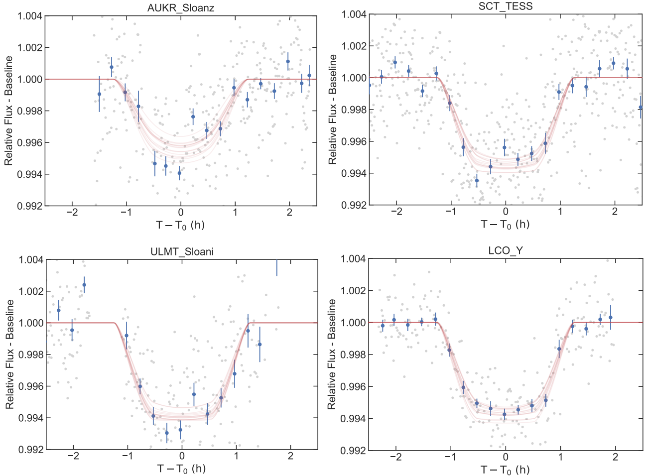
Figure 4. Same as Figure 3, but showing the observations taken with AUKR, SCT, ULMT, and LCO.
