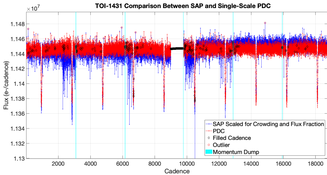
Figure 16. TESS Sector 15 photometry of TOI-1431 from the SAP (blue points) and single-scale MAP PDC (red points) light curves. The SAP light curve shows ‘whisker’-like flux dips that are caused by brief spacecraft pointing excursions, some of which overlap with the transit events. The correction applied to the single-scale MAP PDC light curve from the use of the Co-trending Basis Vectors has removed these features.
