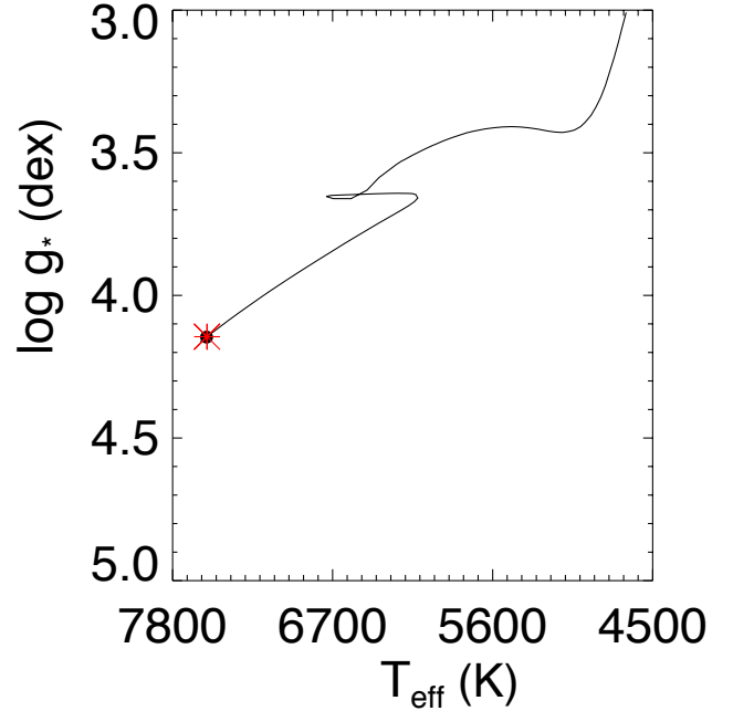
Figure 8. The YY mass track for TOI-1431. The black line represents the mass track interpolated at the model values for M_{\star} , [\text{Fe}/\text{H}] , and age. The black circle is the best-fit model value for T_{\text{eff}} and \log g while the red asterisk is the best-fit model age along the track. The black circle and red asterisk almost perfectly overlap indicating excellent consistency among all the components of the global model.
