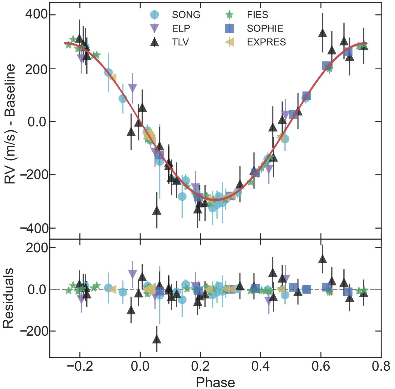
Figure 5. Radial velocity measurements of TOI-1431 b/MASCARA-5 b as a function of orbital phase. The radial velocities from SONG, NRES (ELP and TLV), FIES, SOPHIE, and EXPRES are represented by the cyan colored circles, purple triangles pointed down, black triangles pointed up, green stars, blue squares, and gold triangles pointed to the left, respectively. A random selection of 20 radial velocity curves drawn from the posterior of the Nested Sample modeling are plotted as the red lines. The bottom panel shows the residuals between the data and the best-fit (posterior median) model.
