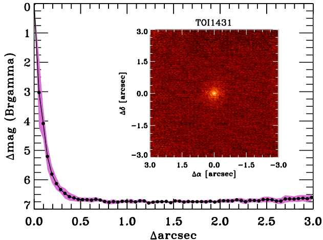
Figure 6. The 5\sigma detection sensitivity and AO image from Keck II NIRC2 high angular resolution imaging of TOI-1431 in the Brgamma-band. The orientation of the AO image has North pointed up and East to the left. No stars were detected within 3'' of TOI-1431.
