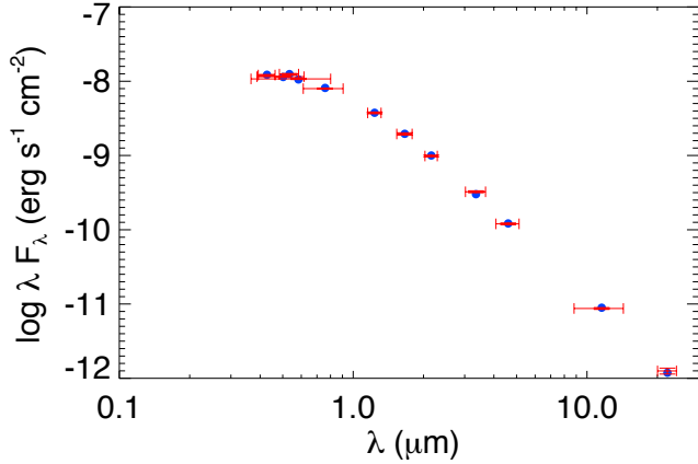
Figure 7. The SED for TOI-1431. The red symbols are the broadband photometric measurements used in the SED analysis (provided in Table 1) with the horizontal uncertainty bars representing the effective width of the passband. The blue symbols are the model fluxes from the best-fit Kurucz atmosphere model.
