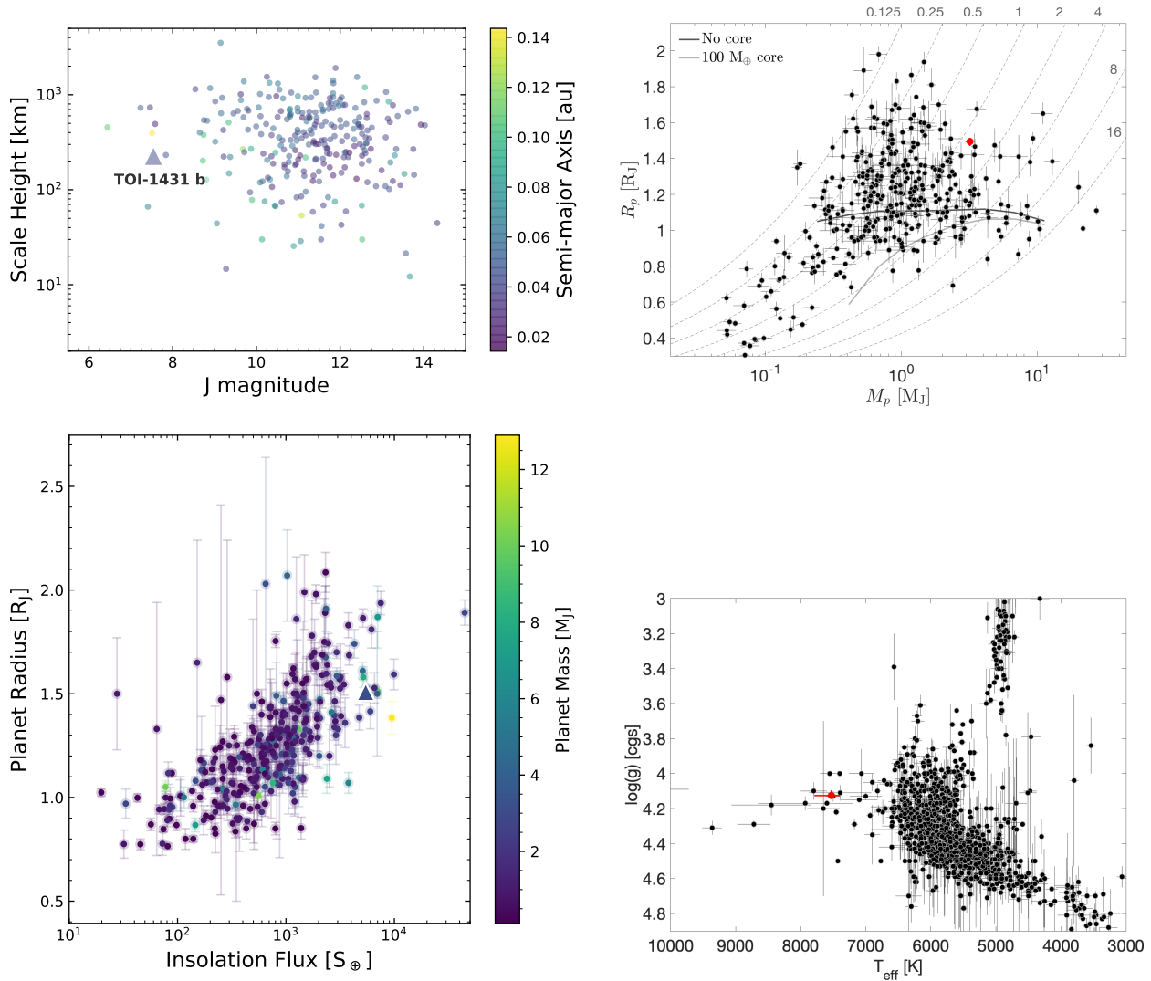
Figure 13. Comparison of TOI-1431 b and its host star with other hot and ultra-hot Jupiter systems. Top left: The atmospheric scale heights of hot Jupiters as a function of host star brightness in the Jmag. The points are colored based on the distance from the host star, with TOI-1431 b plotted as a triangle. This planet transits one of the brightest stars, making it an excellent candidate for future follow-up atmospheric studies. Top right: Planet mass versus radius of hot Jupiters. The red point is the location of TOI-1431 b. Planets located above the dark grey solid line are predicted to have no solid core while those plotted below the light grey solid line are predicted to have a solid core of at least 100 M ⊕ (Fortney et al. 2007). The dotted lines are isodensity lines, with the density value given in the top-left, in cgs units. This plot shows that TOI-1431 b is moderately inflated compared to other Jovians of similar mass. Bottom left: Incident stellar irradiation versus planet radius for all known Jovians and sub-Jovians that have measured masses and radii with the planet masses indicated by the color scale on the left. TOI-1431 b is plotted as the colored triangle on the right and it is clear that this planet is one of the most highly irradiated planets. Bottom right: Plot of stellar effective temperature versus surface gravity for planet hosting stars. TOI-1431 is plotted as the red point and shows that it is one of the hottest (top 1%) known planet hosting stars.
