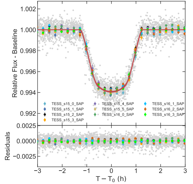
Figure 15. Phase-folded and detrended light curve of TOI-1431 from the simultaneous hybrid cubic spline detrending model using the SAP data. The colored points represent the individual phased light curve segments across Sectors 15 and 16 that have been binned at a cadence of 15 m. The red solid lines are 20 light curve models drawn from the posteriors of the Nested Sampling analysis in Allesfitter .
