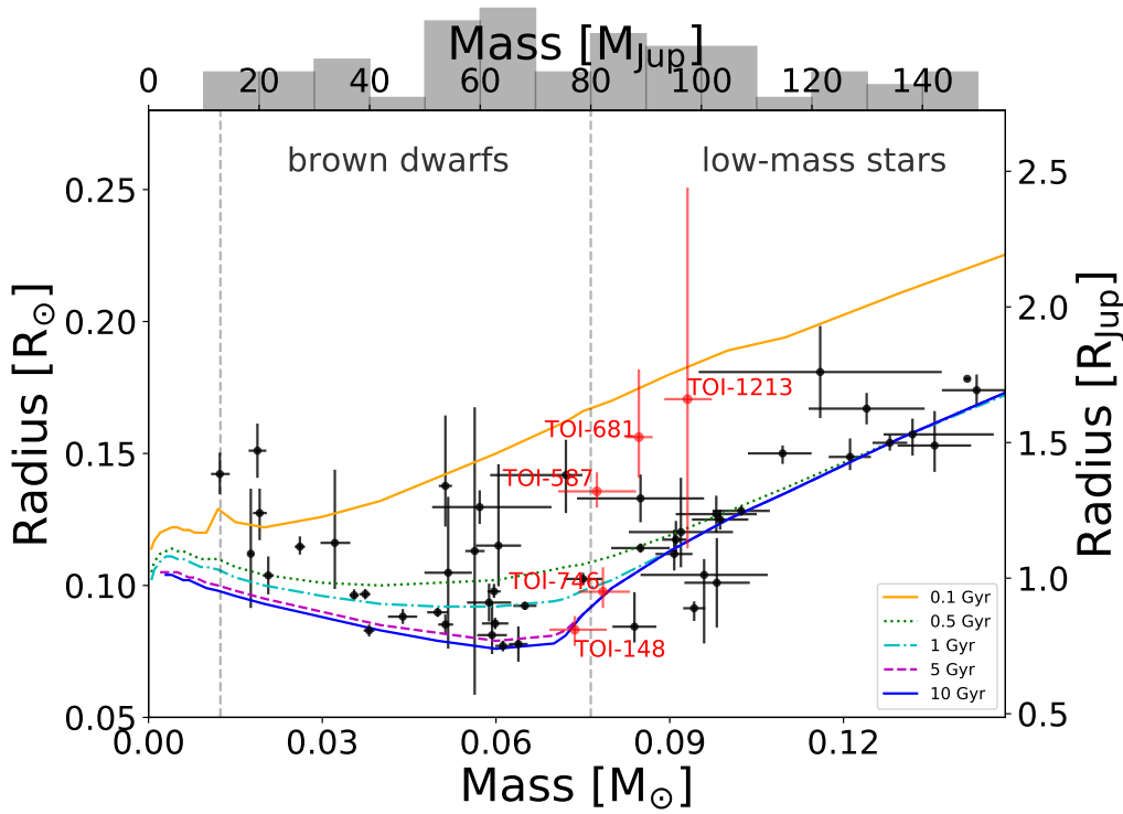
Fig. 10. Radius-mass diagram for the 54 brown dwarfs and low-mass stars presented in Table 4. The five companions presented in this work are highlighted in red. The gray vertical dashed lines display the 13 and 80 M_{\text{Jup}} approximate boundaries of the brown dwarf regime. The colored lines display isochrone models from Baraffe et al. (2003, 2015) for low mass stars and substellar objects at solar metallicity with ages of 0.1, 0.5, 1, 5, and 10 Gyr. The histogram at the top displays relative occurrence of these transiting objects. We note the brown dwarf RIK 72b is not shown because its radius is 3.1 R_{\text{Jup}} .
