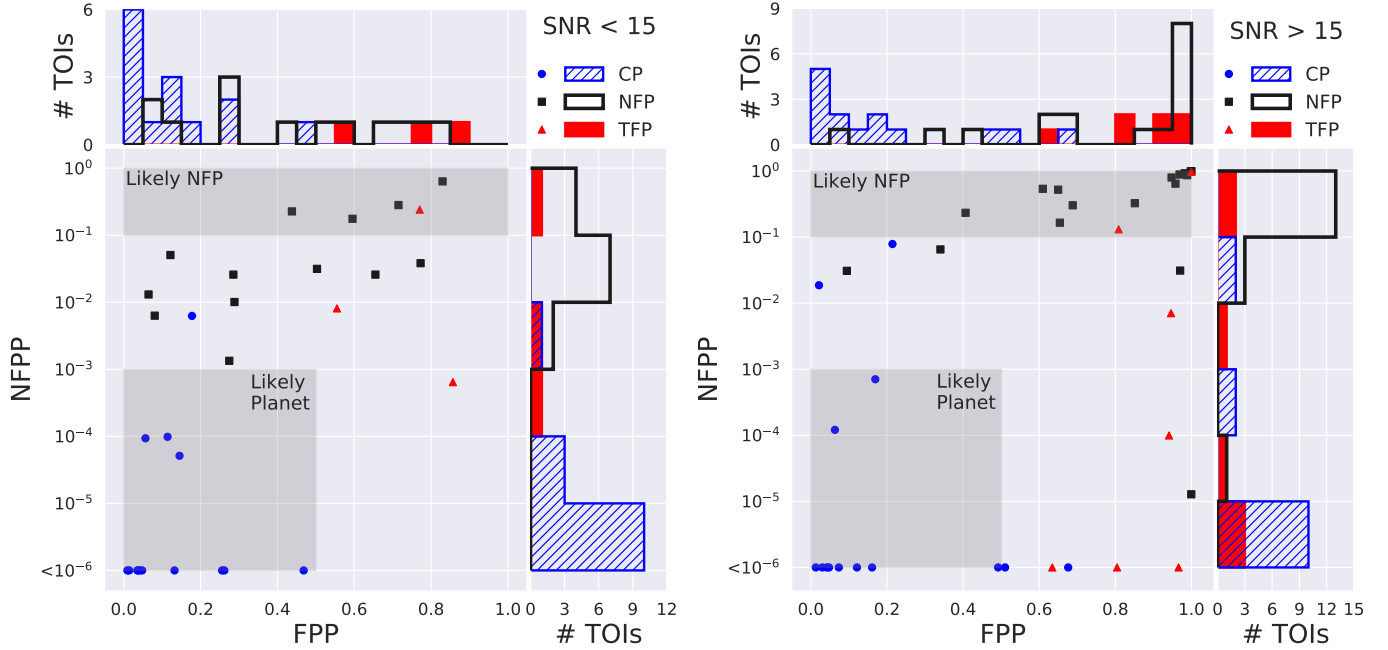
Figure 12. NFPP vs FPP for SNR < 15 (left) and SNR > 15 (right). We designate TOIs with \text{NFPP} < 10^{-3} and \text{FPP} < 0.5 as likely planets. For TOIs with \text{NFPP} < 10^{-3} , and \text{FPP} \leq 0.01 , we are able to rule out FPs with a high enough confidence to consider them validated. Lastly, we are able to identify TOIs that are NFPs with high confidence when \text{NFPP} > 10^{-1} .
