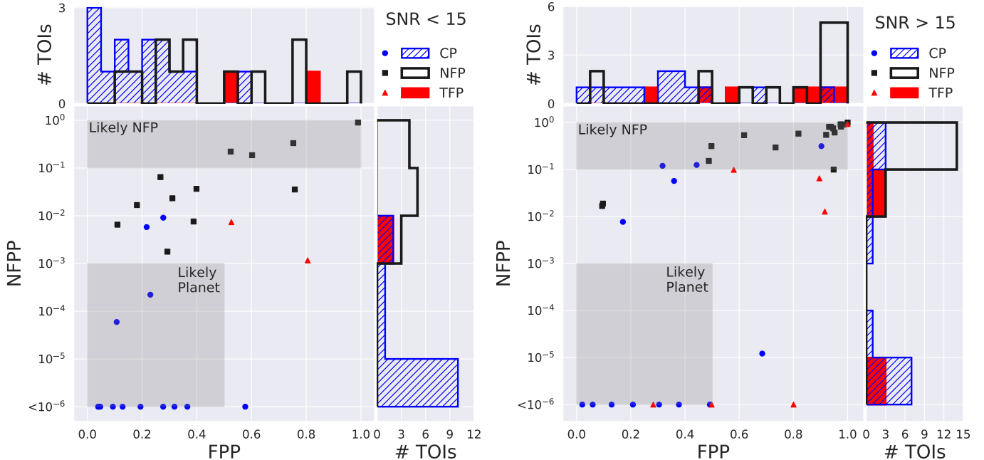
Figure 15. NFPP vs FPP for SNR < 15 ( left ) and SNR > 15 ( right ), but calculated using 30-minute cadence TESS data. While we are unable to identify a region in which we can validate TOIs, we can still designate TOIs with NFPP < 10^{-3} and FPP < 0.5 as likely planets. Additionally, we are still able to identify TOIs that are NFPs with high confidence when NFPP > 10^{-1} .
