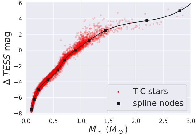
Figure 4. \Delta TESS magnitude between a star of mass M_* and a 10th magnitude, 1M_\odot star. Red points are stars queried from the TIC located between 99 – 101 pc away. Black squares are the nodes of the spline relation used to calculate the TESS mag of unresolved stars modeled in our calculations.
