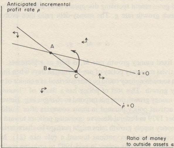
Figure 2. Adjustment Dynamics When a Fall in the Expected Incremental Profit Rate \hat{q} from an Initial Equilibrium at A Leads Finally to a Return to Steady-State.
