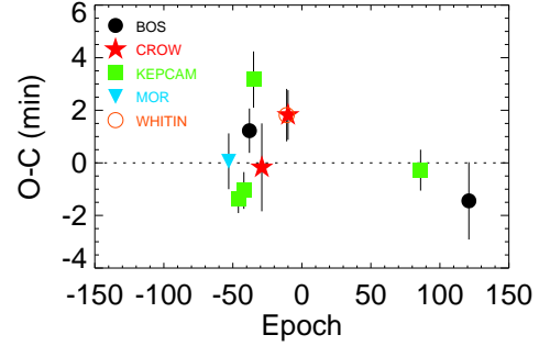
Figure 10. The residuals of the transit times from the best-fit ephemeris. The transit times are given in Table 3. The WHITIN observations at epoch -13 are hidden behind the CROW observations at epoch -12.
