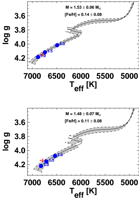
Figure 11. Theoretical HR diagrams based on Yonsei-Yale stellar evolution models (Demarque et al. 2004). The solid lines represent the evolutionary tracks for the best-fit values of the mass and metallicity of the host star from the global fits using the Yonsei-Yale constraints (top panel) and the Torres constraints (bottom panel) as described in Section 3.5. The tracks for the extreme range of 1\sigma uncertainties on M_* and [\text{Fe}/\text{H}] are shown as dashed lines, bracketing the 1\sigma range shown in grey. The red crosses show T_{\text{eff}} and \log g from the EXOFAST global fit analysis. The blue dots represent the location of the star for various ages in Gyr. We adopt the Yonsei-Yale constrained global fit represented in the top panel resulting in an estimated age of 1.3 \pm 0.2 Gyr, where we note the uncertainty does not include possible systematic errors in the adopted evolutionary tracks.
