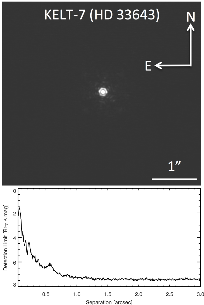
Figure 5. Top: Br- \gamma AO image for KELT-7 (HD 33643) in Br- \gamma ( \lambda = 2.1654 mm). North is up, east is left. The horizontal bar is 1''. No nearby companions or background sources were detected. Bottom: 5 \sigma detection limit as a function of angular separation. Detection limits at 0.1'', 0.2'', 0.5'', and 1.0'' are also given in Section 2.4.
