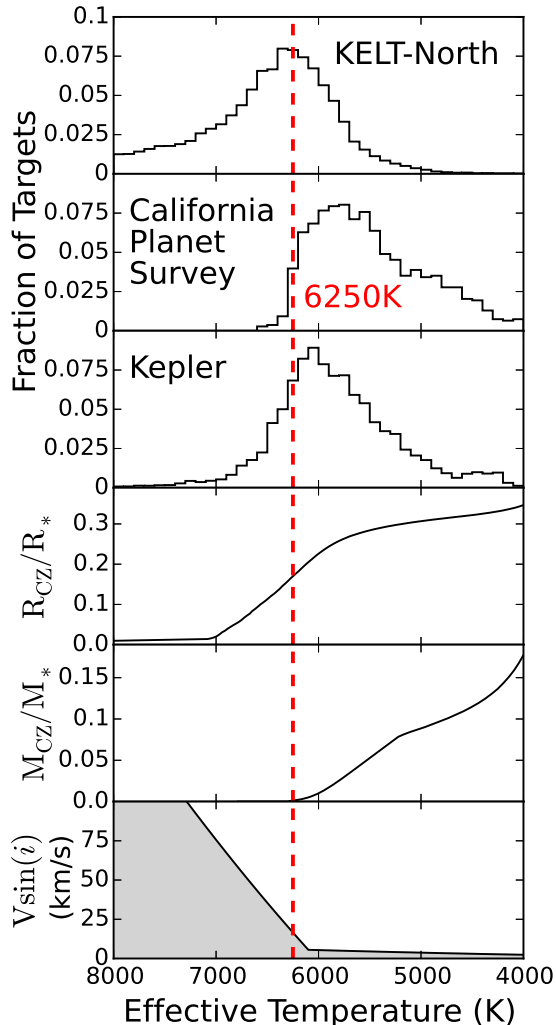
Figure 1. The top three panels show the effective temperature distribution for the stars targeted by the KELT-North transit survey (Sivervd et al. 2012), the California Planet Survey (CPS) radial velocity (RV) search (Wright et al. 2004), and the Kepler mission (stars observed for all 16 quarters and with \log g > 4.0 according to Kepler Q1-Q16 Stellar Parameters Database a ). The fourth and fifth panels from the top show the relative depth and mass of outer stellar convective zones at these temperatures (van Saders & Pinsonneault 2012), while the sixth, bottom, panel shows the observed stellar v \sin i distribution (Reiners & Schmitt 2003). The red dashed line at 6250K shows the approximate location of the Kraft Break (Kraft 1970).
