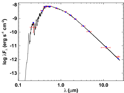
Figure 12. Measured and best-fit SED for KELT-7 from UV through mid-IR. The red error bars indicate measurements of the flux of KELT-7 in UV, optical, NIR, and mid-IR passbands and listed in Table 2. The vertical bars are the 1\sigma photometric uncertainties, whereas the horizontal error bars are the effective widths of the passbands. The solid curve is the best-fit theoretical SED from the NextGen models of Hauschildt et al. (1999), assuming stellar parameters T_{\text{eff}} , \log g , and [\text{Fe}/\text{H}] fixed at the adopted values in Table 4, with A_V and d allowed to vary. The blue dots are the predicted passband-integrated fluxes of the best-fit theoretical SED corresponding to our observed photometric bands. The 22 micron band shows a slight IR excess as discussed in Section 3.7.
