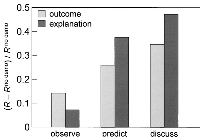
Fig. 1. Improvement in rate R of correct outcomes (light gray) and explanations (dark gray) for each mode over the no demonstration (control) group, normalized to the rate for the control group.
