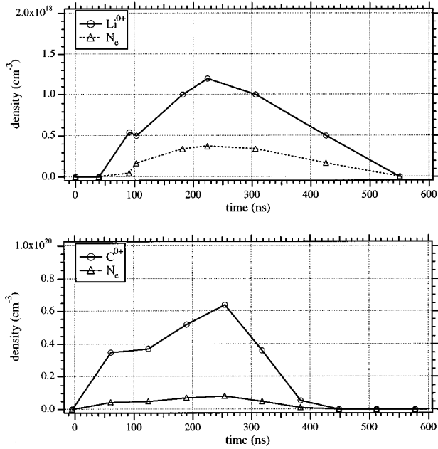
FIG. 2. Electron and neutral atom densities as a function of time measured for lithium and carbon targets. Lithium data: intensity of ablating laser pulse on target is 3 \times 10^8 W/cm 2 ; probe beam is 250 \mu m from the target surface. Carbon data: intensity of ablating pulse on target is 1 \times 10^9 W/cm 2 ; probe beam is 0 \mu m from the target surface.
