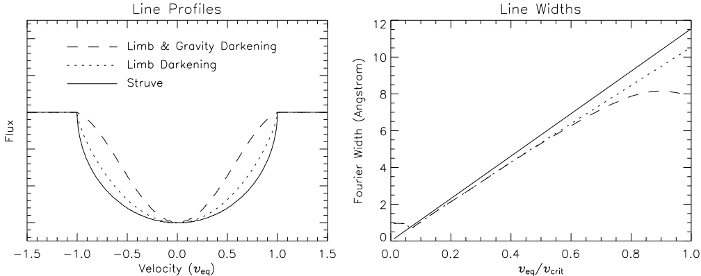
Figure 2. Left: Direct comparison of the three types of line profile – Struve, limb darkened, and gravity-darkened plus limb darkened – shown in Fig. 1. Note the progression to a narrower line as each subsequent effect is included. Right: The Fourier line width as a function of v_{\text{eq}}/v_{\text{crit}} , for the three models. The width data for the non-Struve models are based on NLTE line synthesis calculations for He I 4471 Å.
