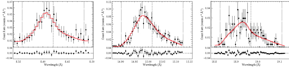
FIGURE 2. In these three panels are three separate emission lines from the Chandra spectrum of the massive star \zeta Puppis. These are, from left to right, the \text{Ly}\alpha line of \text{Mg XII} at 8.42 Å, the \text{Fe XVII} line at 15.01 Å which is the 3d^1P_1 level to the ground state, and the \text{Ly}\alpha line of \text{O VIII} at 18.97 Å. The laboratory rest wavelengths for each emission line are indicated by the vertical dashed lines while the Doppler shifts associated with the stellar wind terminal velocity are represented by the light dashed vertical lines. The data are the points with (Poisson) error bars, the model is shown as the solid (red) histogram, and the fit residuals are shown in the horizontal windows below each data plot. The values of R_0 , the onset radius of x-ray emission we find for each line, are R_0 = 1.34^{+0.22}_{-0.17} R_* , 1.55^{+0.13}_{-0.12} R_* , and 1.18^{+0.41}_{-0.17} R_* for the Mg, Fe, and O lines, respectively. This is consistent with the predictions of the LDI wind-shock model, in which strong shocks start to form several tenths of a stellar radius above the photosphere. The values we derive for the \tau_* parameter from the profile model fitting are \tau_* = 1.22^{+0.53}_{-0.45} , 1.94^{+0.32}_{-0.33} , and 3.02^{+0.52}_{-0.57} . Note that these values are consistent with the wavelength dependence of the atomic opacity of the wind, as expected.
