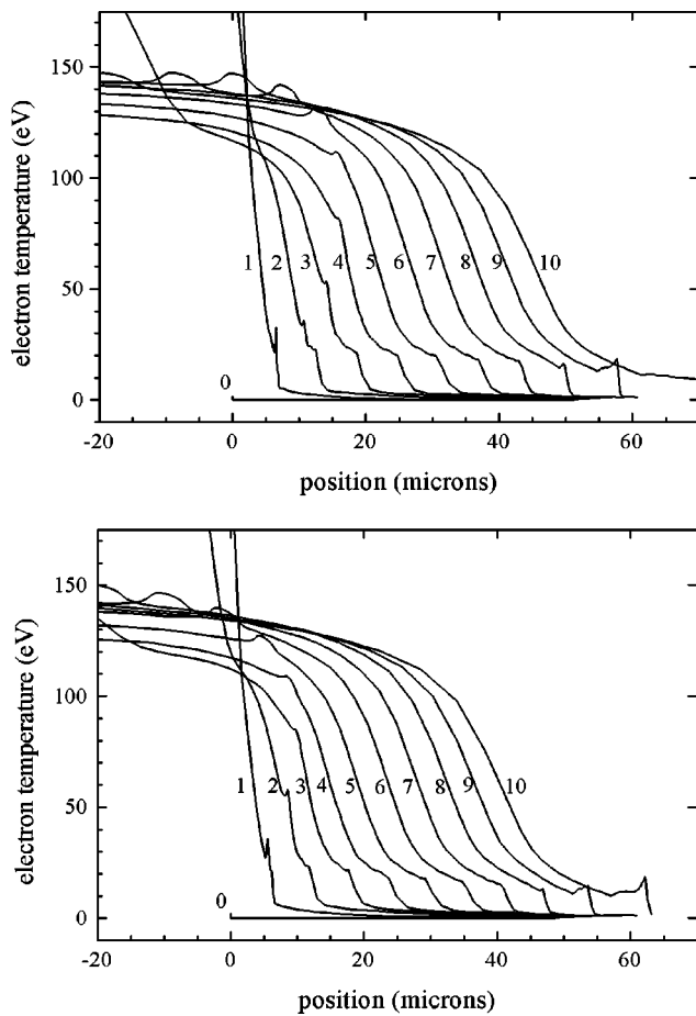
FIG. 7. Hydrodynamics simulations of the undoped (top) and doped (bottom) samples, with the temperature profiles shown at 11 different times, from t=0 to t=1 ns. Each time is labeled in units of 100 ps. Note that the Marshak wave velocity is slower in the doped sample. A shock wave, moving ahead of the radiation wave, is visible in the simulations. The location of the tracer layer can be discerned, as the tracer is slightly hotter than the surrounding plastic. Finally, note the hot ablated plasma on the left (radiation is from the left). At early times it is especially hot due to the deposition of scattered laser light onto the ablator sample.
