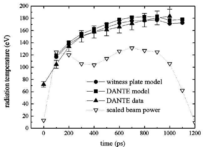
FIG. 6. Results of view-factor simulations of our OMEGA halfracum experiments. The filled squares are the simulated DANTE temperatures and the filled triangles are the measured DANTE temperatures. The filled circles are the calculated time-dependent drive temperature onto the sample, which is used as input to the subsequent hydrodynamics models. We also show the (scaled) laser beam powers from shot 19 526.
