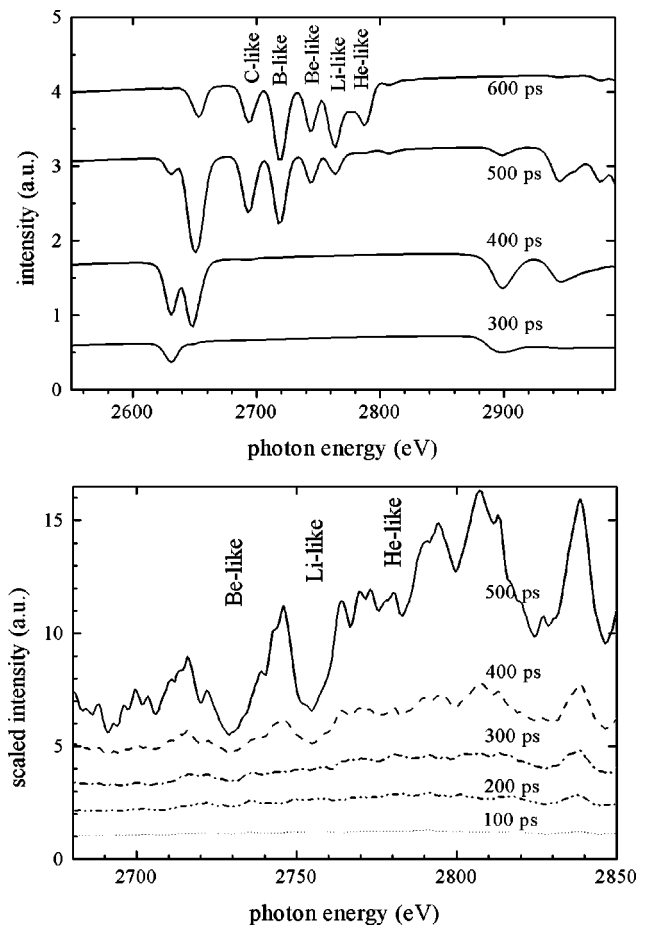
FIG. 8. Spectral simulations postprocessed from the hydrodynamics simulations shown in Fig. 7 (top) and the LXS data from shot 19 526 (bottom), with the undoped target and a tracer depth of 6.3 \mu\text{m} . Note that the x -axes ranges are different in the model and data plots.
