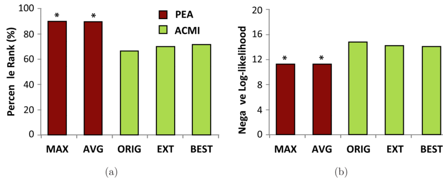
Fig. 5. Accuracy of inference solutions. In (a), the percentile rank of the true solution's probability is shown. In (b), the negative log-likelihood of the true solution is shown. Lower scores mean a higher probability value for the correct answer. In both, columns are the average score over all amino acids in all test-set proteins. Dark (red) bars represent variations of PEA, while light (green) bars represent variations of ACMI. *denotes a statistically significant difference with ORIG at p < 0.01 .
