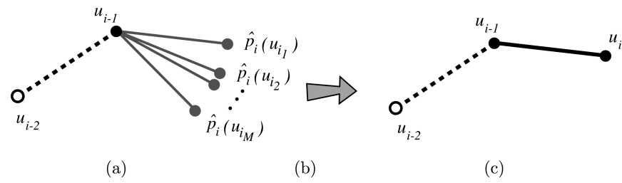
Fig. 4. ACMI's Phase 3 sampling step for amino acid i . In (a) Phase 3 samples M possible new locations, u_{i_m} . In (b) these locations are weighted by their agreement with the Phase 2 probability, \hat{p}_i . In (c) one location is chosen from the weighted distribution to be amino acid i 's location, u_i .
