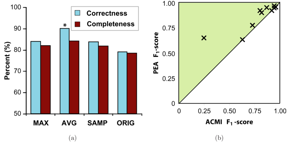
Fig. 6. Protein-structure prediction accuracy. In (a), we show correctness (light blue) and completeness (dark red) of PEA. *indicates statistically significant difference compared to ORIG at p < 0.05 . In (b) we show a detailed comparison of F_1 -scores for ACMI ( x -axis) and PEA using the averaging aggregator ( y -axis). Each point represents one protein and the shaded region indicates better scores for PEA.
