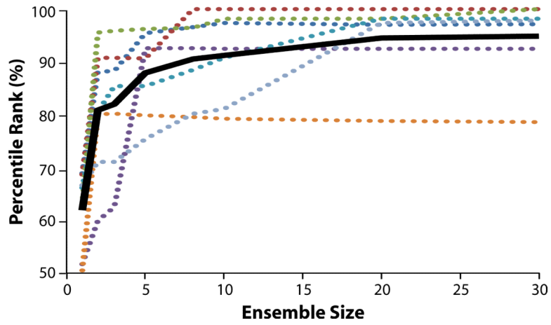
Fig. 7. Learning curve for ensemble inference. Each dashed line represents one protein's percentile scores for Phase 2 posteriors as the number of ensemble components increases. The solid black line represents the average learning curve.
