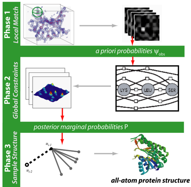
Fig. 2. The three-phase ACMI pipeline. Given an electron-density map and protein sequence, Phase 1 performs a local-match search independently for each amino acid. Phase 2 combines these results with global constraints to create posterior probabilities of each amino acid's location. Finally, Phase 3 uses these marginals to sample physically feasible, all-atom protein structures. The box on the right in Phase 2 shows a portion of an MRF for an example protein sequence.
