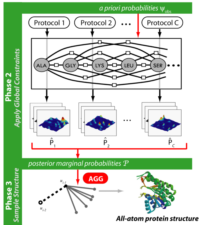
Fig. 3. Probabilistic Ensembles in ACMI (PEA). Phase 1 (omitted) is the same as in the ACMI framework (Fig. 2). Phase 2 performs C independent inference runs, each with a unique protocol. This results in a set of C marginal probabilities for each amino acid's location. Phase 3 aggregates the set of marginal probabilities to produce a protein structure.
