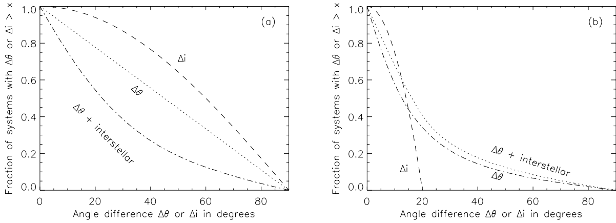
FIG. 2.—Effects of projection in transforming the true distribution of disk orientations \Delta i to the observed distribution of polarization position angle differences \Delta\theta . (a) The cumulative distribution function of a random distribution (i.e., proportional to total solid angle at a given \Delta i ) of angle differences \Delta i is shown as a dashed line. This is projected into a uniform distribution of observed position angle differences \Delta\theta (dotted line). Adding an additional component of interstellar polarization (see § 4.3) gives a distribution of observed \Delta\theta (dot-dashed line) that is more peaked toward small angle differences. (b) The same comparison, but for an input distribution of angle differences \Delta i (dashed line) that is random from 0^\circ – 20^\circ . Projection of the disks into the plane of the sky results in some observed position angle differences \Delta\theta that are much larger than any of the true orientation differences \Delta i (see § 2).
