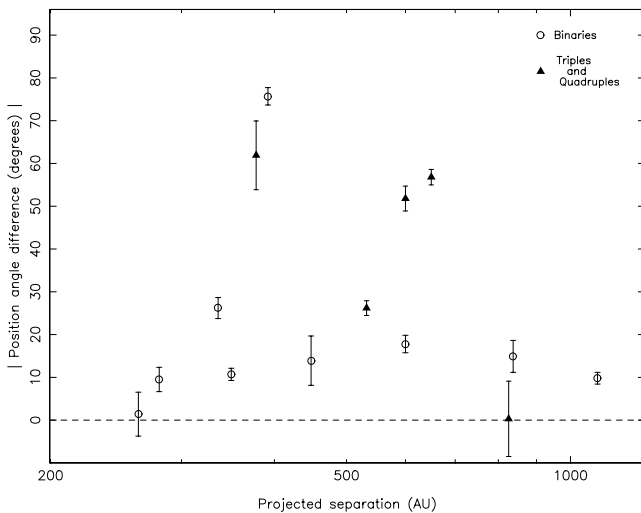
FIG. 1.—Absolute value of the difference in polarization position angles between the two stars in each binary is shown as a function of projected binary separation. Filled triangles show systems that are triple or quadruple. In the majority of the binary systems the two components have similar position angles, indicating that their disks are aligned, while the triple or quadruple systems tend to have more random disk orientations. There is no obvious dependence of alignment on binary separation.
