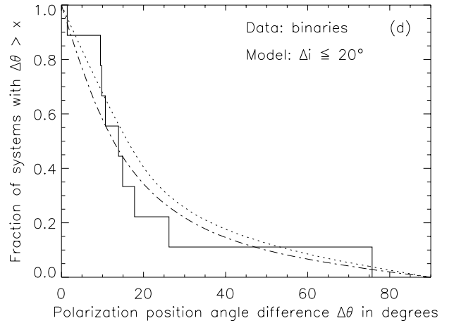
FIG. 3.—Comparison between observed polarization position angle differences and various assumed distributions of angle differences. The cumulative distribution function of the observed polarization position angle differences \Delta\theta ( stepped solid line ), compared with models with a random distribution of disk orientations ( dotted line ), and with a random distribution of intrinsic orientations modified by an overlying component of interstellar polarization ( dot-dashed line ). (a) All data compared with a random distribution. (b) The binaries only, compared to a random distribution. (c) The triples and quadruples (for which only the widest pair is resolved in our observations), compared to a random distribution. (d) The binaries only, compared to a distribution that includes angles only from \Delta i = 0^\circ - 20^\circ . The binaries are inconsistent with (b) a random distribution but are well fitted by (d) the aligned 0^\circ - 20^\circ distribution. In contrast, the triples are well fitted by (c) a random distribution. If interstellar polarization is significant ( dot-dashed lines ), the entire data set is well fitted by (a) a random distribution. See Table 5 for exact confidence levels for the various cases.
