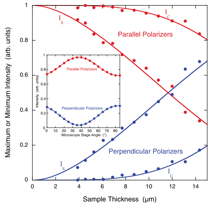
FIG. 7. (Color online) Maximum and minimum intensities as a function of sample thickness for 15 wt% DSCG at 25^\circ\text{C} . The intensities with parallel and perpendicular polarizers start at 1 and 0, respectively, at zero sample thickness. The experimental data are shown as solid circles and the solid lines are fits to the elastic and optical theory as described in the text, yielding best-fit values for \Delta n of -0.0177 and W_\phi/k_{22} of 5.70 \times 10^5\ \text{m}^{-1} , with a determination of W_\phi of (3.4 \pm 0.6) \times 10^{-7}\ \text{J/m}^2 . Inset: intensity as a function of microscope stage angle for a 15 wt% DSCG sample of thickness 7.7\ \mu\text{m} at 25^\circ\text{C} . The fits are to Eq. (5) after 37.3^\circ has been subtracted from each angle value.
