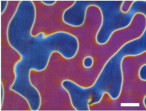
FIG. 6. (Color online) Right- and left-handed twist domains in 15 wt% DSCG using white light, a 5\times objective, parallel polarizers, and a \lambda plate. The thickness of the sample is roughly 10\ \mu\text{m} . The length of the scale bar corresponds to 300\ \mu\text{m} .
