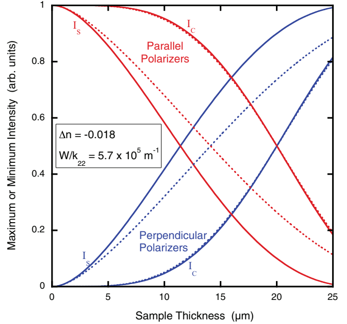
FIG. 5. (Color online) Theoretical maximum and minimum intensities, I_C and I_S , for 633 nm light versus sample thickness with W_\phi/k_{22} = 5.7 \times 10^5 \text{ m}^{-1} and \Delta n = -0.018 . The intensities with parallel and perpendicular polarizers start at 1 and 0, respectively, at zero sample thickness. The solid lines are for the nonchiral case and the dotted lines are for a pitch of 60 \mu\text{m} . The I_C and I_S labels are for a specific definition of the angle \theta in Eq. (5).
