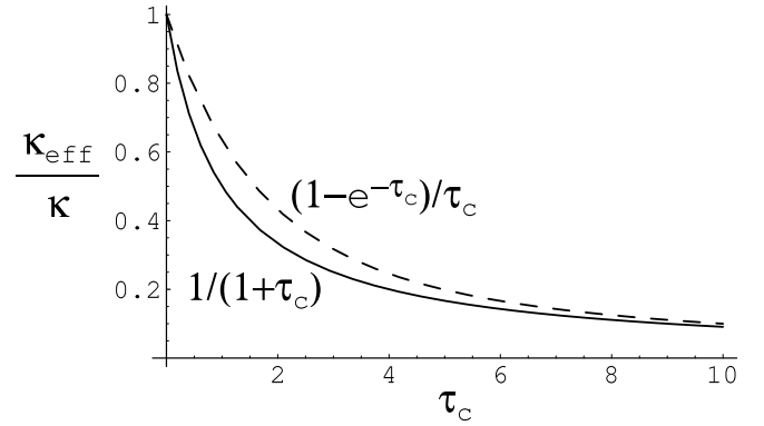
FIG. 1.—Comparison of absorption ( dashed curve ; eq. [4]) and mean path ( solid curve ; eq. [6]) scalings of effective opacity in a porous medium, plotted as a function of clump optical thickness \tau_c .
