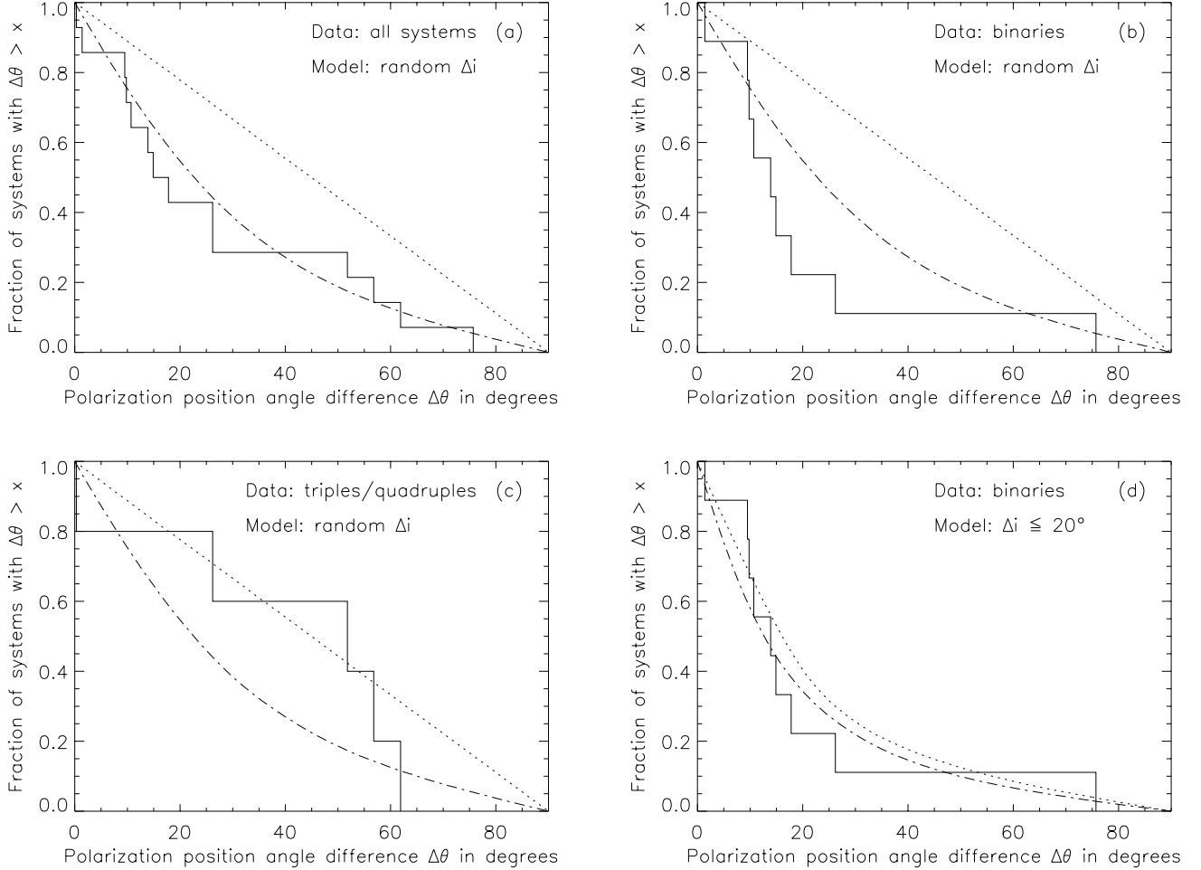
FIG. 3.—Comparison between observed polarization position angle differences and various assumed distributions of angle differences. The cumulative distribution function of the observed polarization position angle differences \Delta\theta (stepped solid line), compared with models with a random distribution of disk orientations (dotted line), and with a random distribution of intrinsic orientations modified by an overlying component of interstellar polarization (dot-dashed line). (a) All data compared with a random distribution. (b) The binaries only, compared to a random distribution. (c) The triples and quadruples (for which only the widest pair is resolved in our observations), compared to a random distribution. (d) The binaries only, compared to a distribution that includes angles only from \Delta i = 0^\circ - 20^\circ . The binaries are inconsistent with (b) a random distribution but are well fitted by (d) the aligned 0^\circ - 20^\circ distribution. In contrast, the triples are well fitted by (c) a random distribution. If interstellar polarization is significant (dot-dashed lines), the entire data set is well fitted by (a) a random distribution. See Table 5 for exact confidence levels for the various cases.
